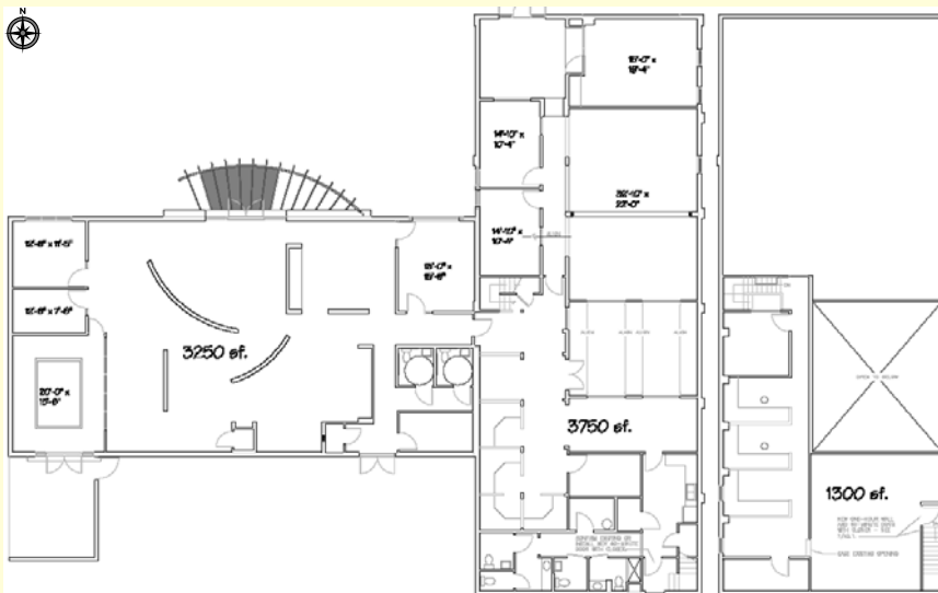
Floor Plan
